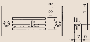
Stichplatte / Throat plate: 91-150 884-24/001
