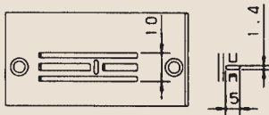
Stichplatte / Throat plate: 91-150 884-24/001
