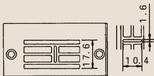
Stichplatte / Throat plate: 91-150 872-24/002
